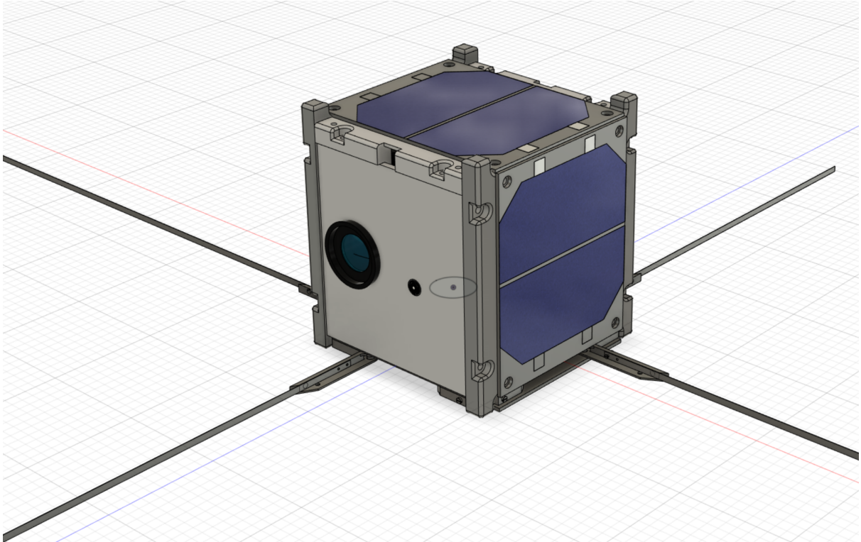
Monopole Antenna x2 with ground elements x2
